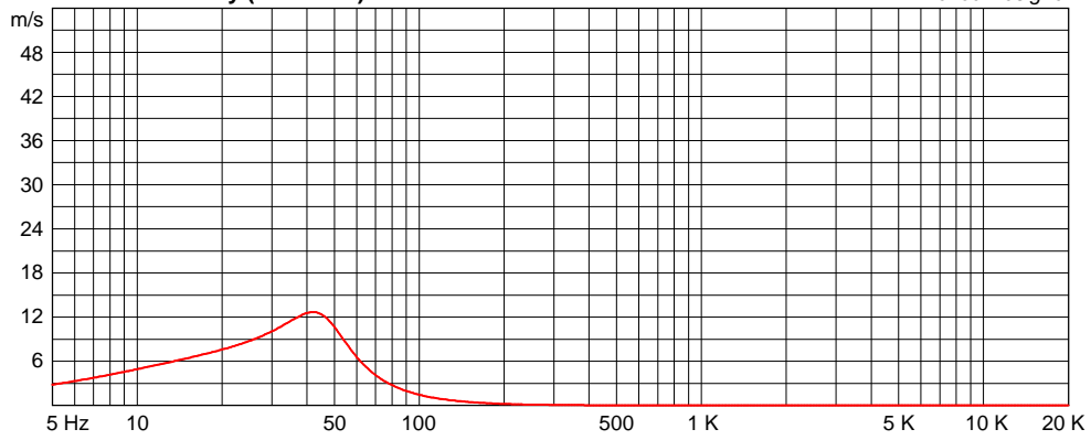
Vent Air Velocity (m/sec/Hz) with 700 watts
