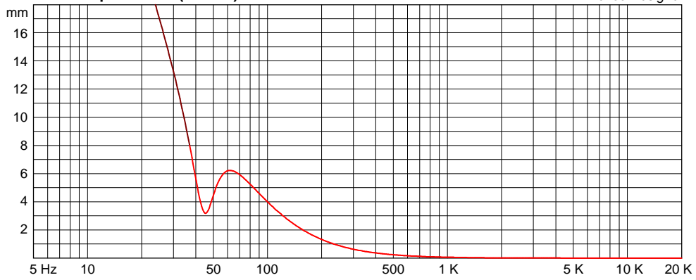
Cone Displacement (mm/Hz) with 700 watts
